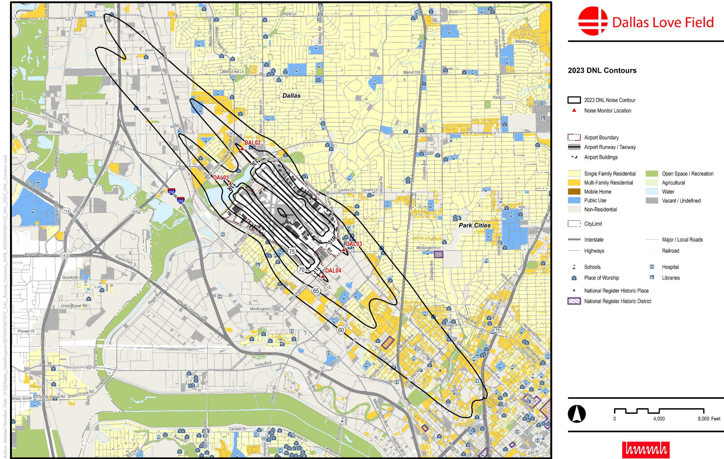
Figure 14. Dallas Love Field 2023 Noise Contour
