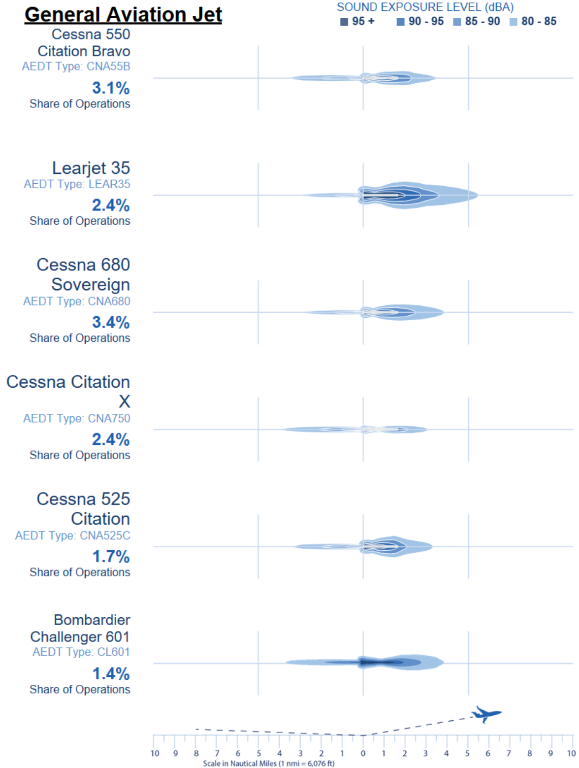
Figure 4. SEL Contours - General Aviation Jets
