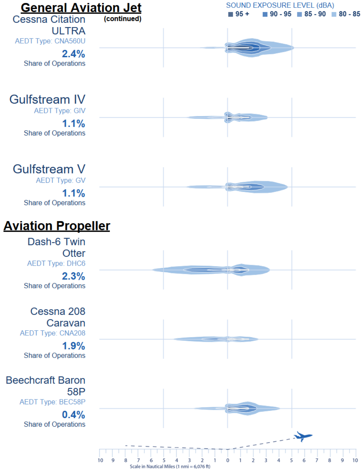
Figure 5. SEL Contours - General Aviation Jets (cont'd) and Propellers
