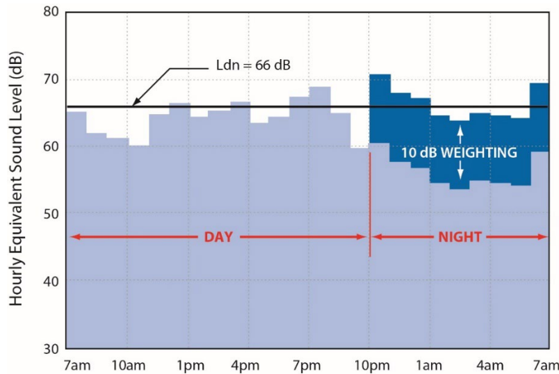
Figure A-6. Example of a Day-Night Average Sound Level Calculation Source: HMMH
