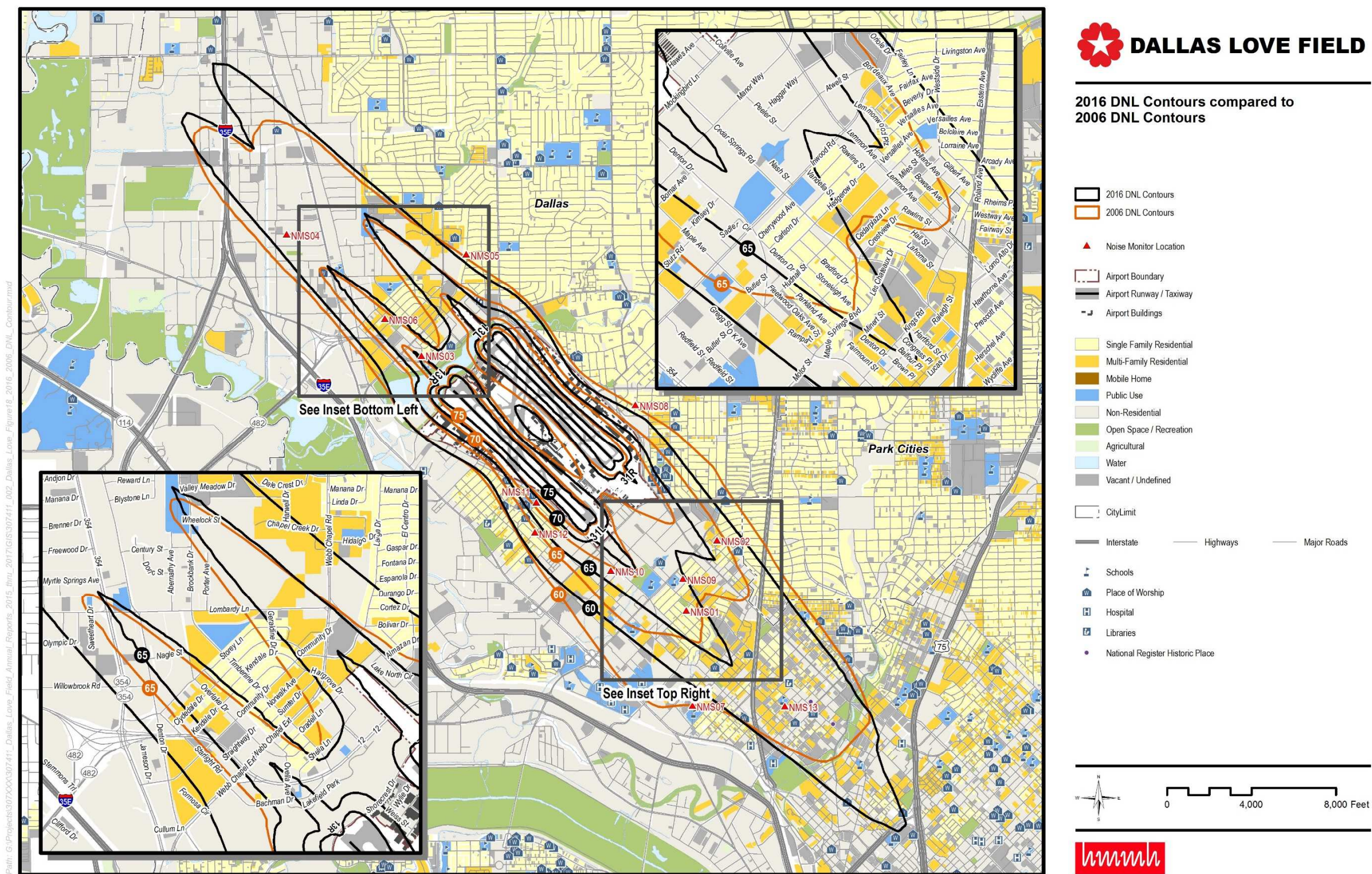
Figure 18 2016 DNL Contours compared to 2006 DNL Contours
